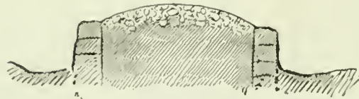
(Fig. 12 a ) Section of Roman Way across Mekro Polje.
